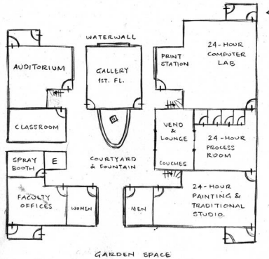
Figure 5581-1. Plan of first floor
