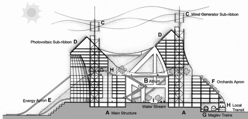
Figure 743-5. Depending on regional climatic and topographical conditions, the Lean Linear City - Arterial Arcology introduces alternative energy production options: continuous arrays of photovoltaic modules harvesting solar energy and a series of windmills capturing wind energy. (Image credit: Cosanti Foundation)
