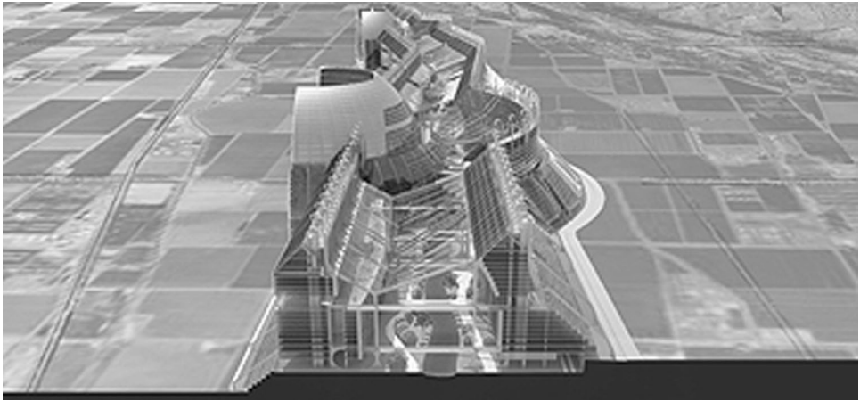
Figure 743-4. The most promising effect of the arterial arcology is a network of logistically distributed habitats capable, in time, of cleansing the land by substantially reducing an enormous fossil fuel dependence, thus restoring ecosystems and enriching the life of the countryside now under the threat of endless sprawl (the City of Phoenix Syndrome). (3D rendering - Youngsoo Kim)
