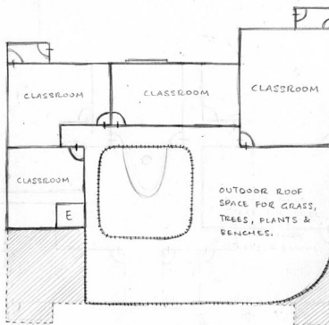
Figure 5582-1. Plan of second floor
